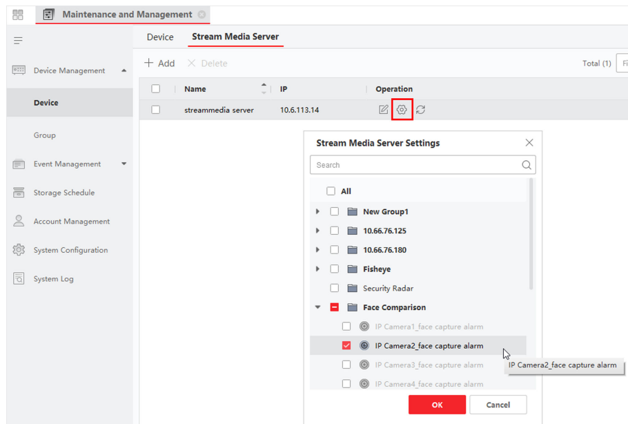
Figure 13-4 Add Cameras to Stream Media Server
