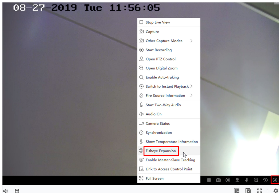
Figure 6-13 Live View in Fisheye Mode
