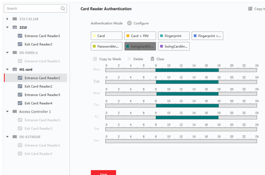
Figure 19-10 Set Authentication Modes for Card Readers
